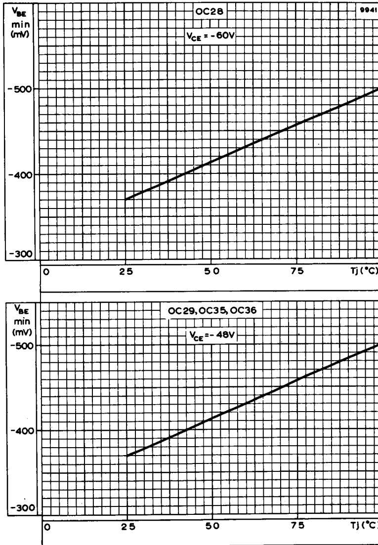
VARIATION OF V_{BE} WITH JUNCTION TEMPERATURE
